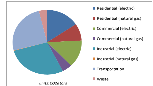
Figure 74: GHG Inventory 2009
