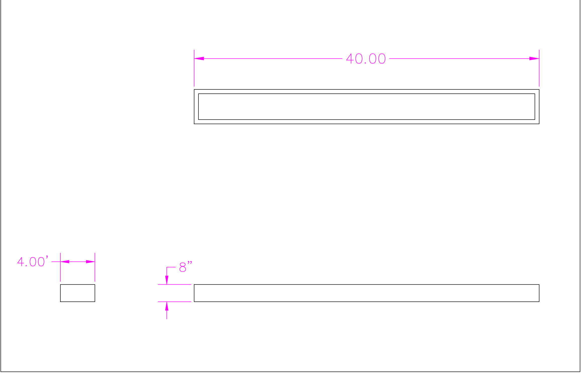
PLANTER DETAIL (TOP, SIDE, FRONT)
