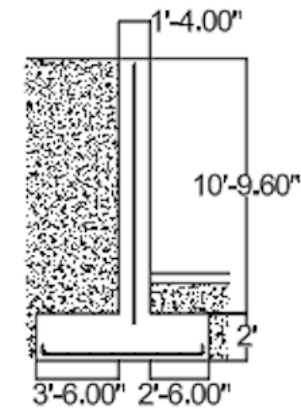
Multi-Use Lodge Load Bearing Wall
