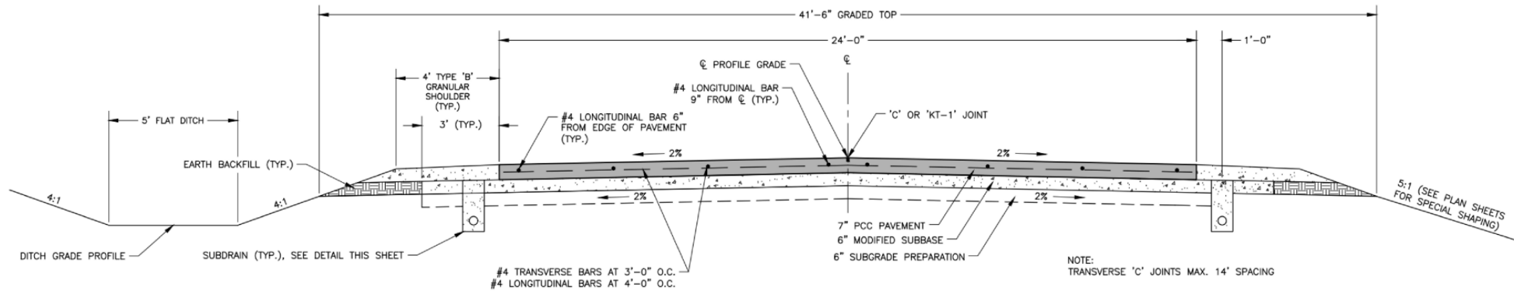
PARK ROAD (STA. 00+00 TO 13+98.47) TYPICAL SECTION 24' PCC PAVEMENT
