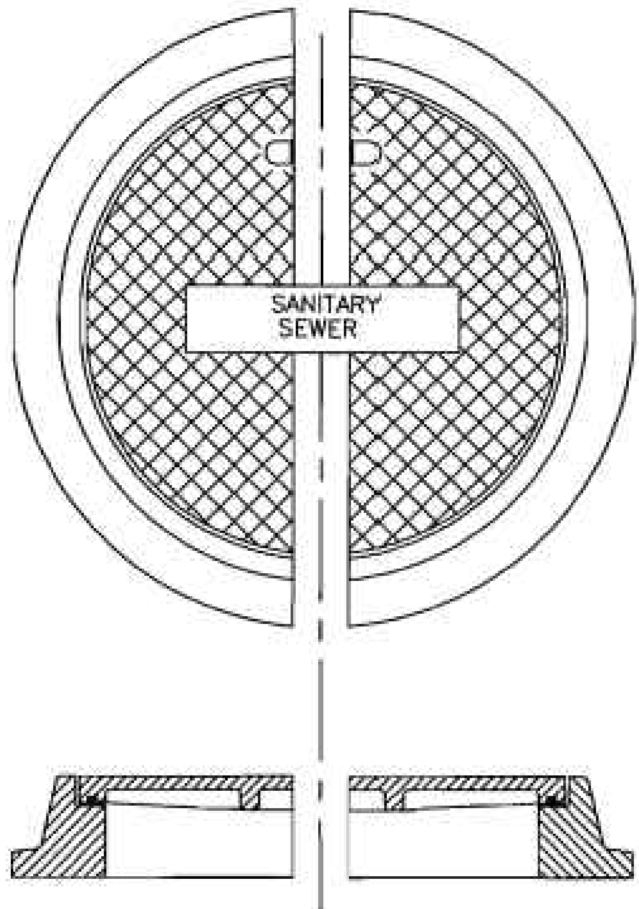
FRAME AND COVER DETAIL
