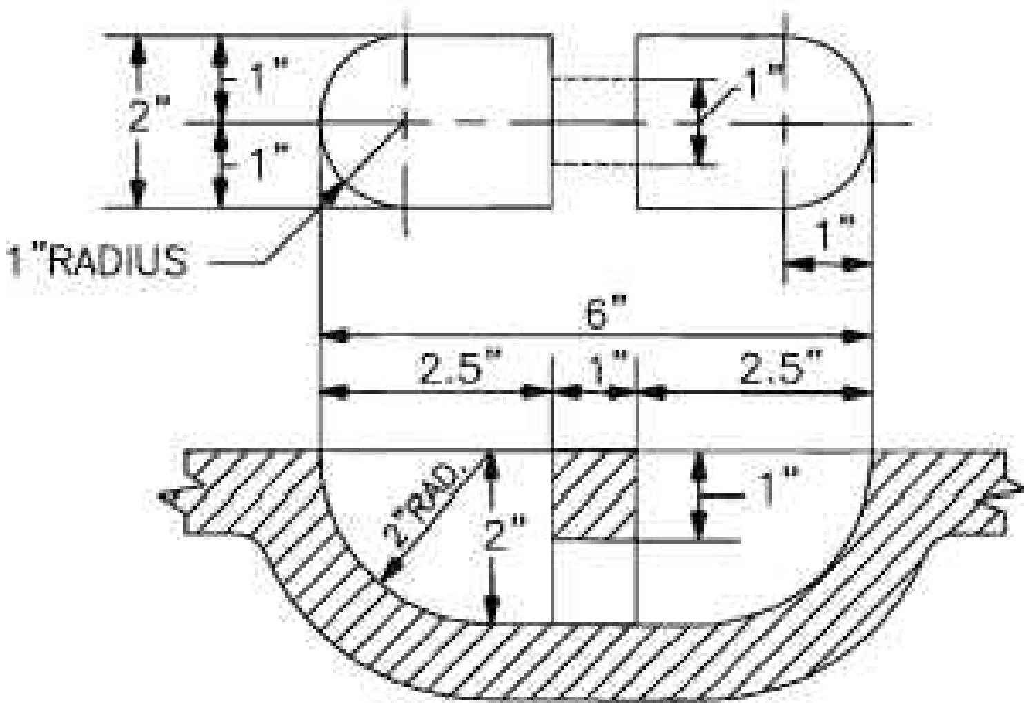
LIFTING RECEPTACLE DETAIL
