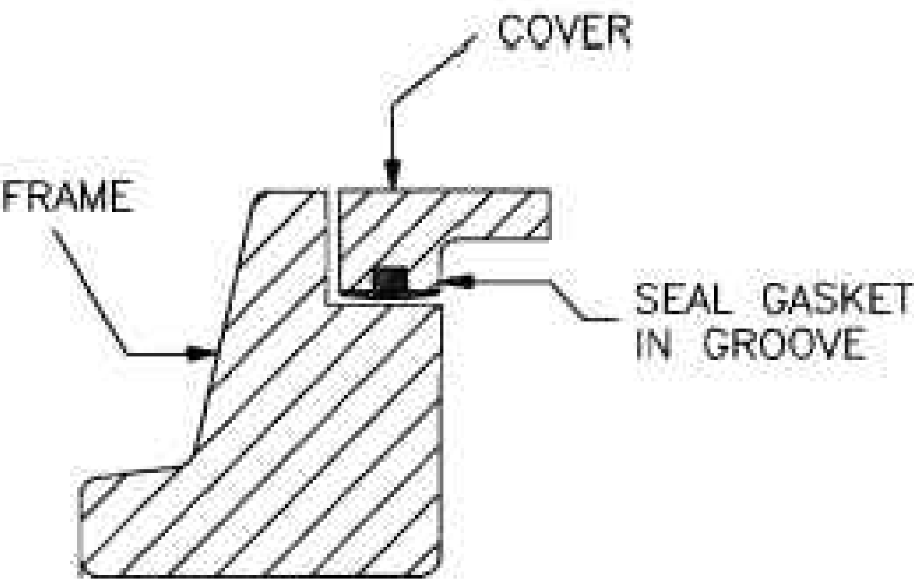
SEAL DETAIL
