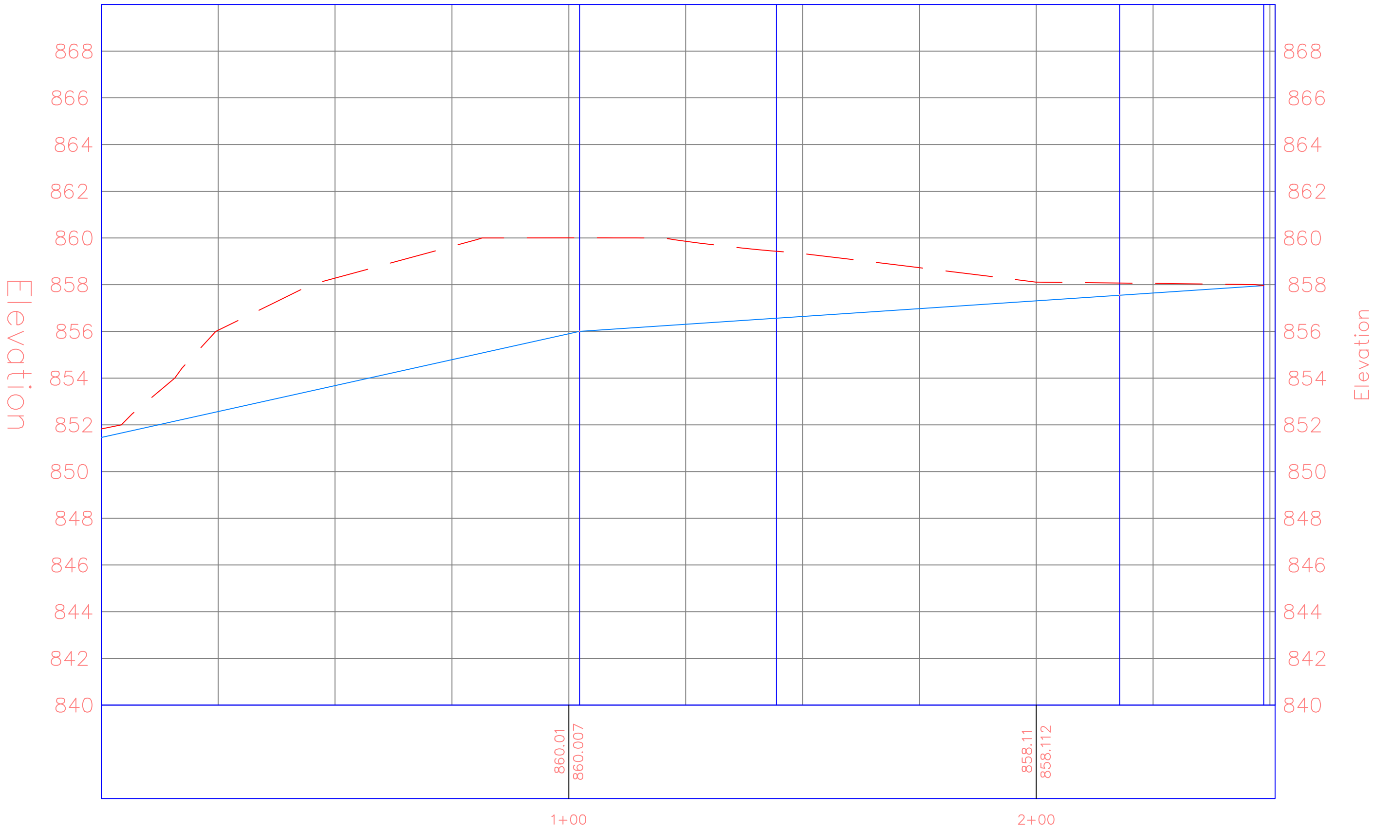
MUP to Parking Existing Shelter PROFILE MUP to Parking Existing Shelter51
