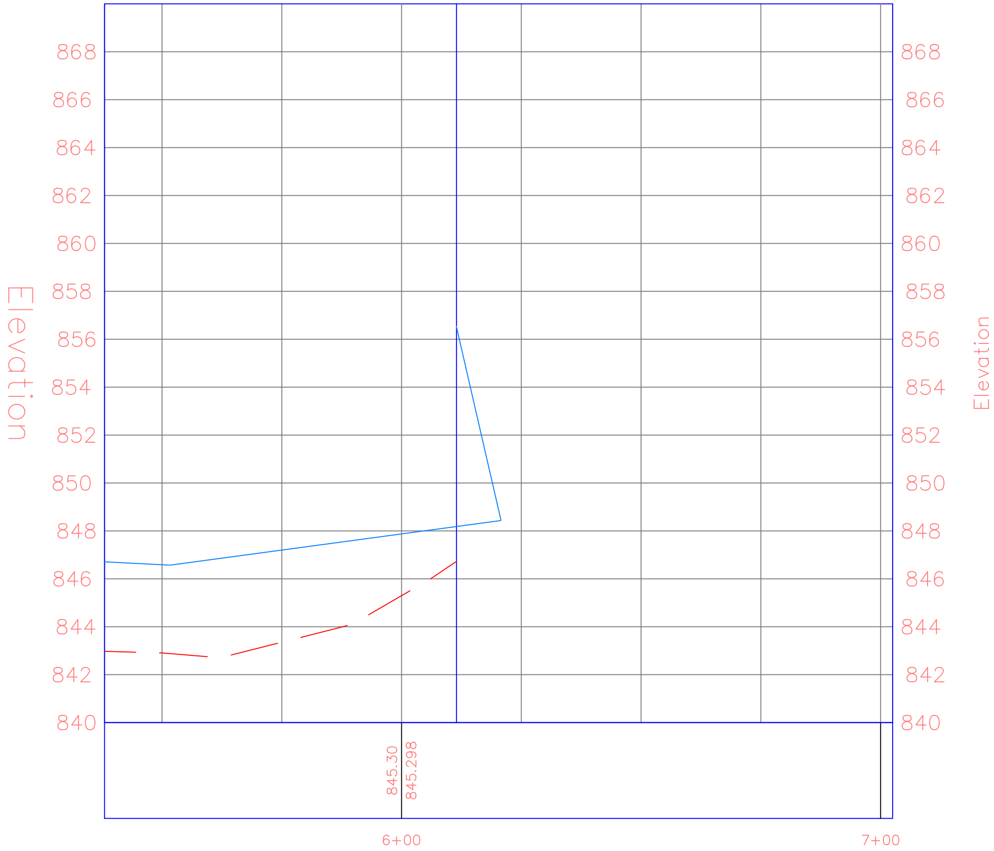
Gravel Path East Alt71
