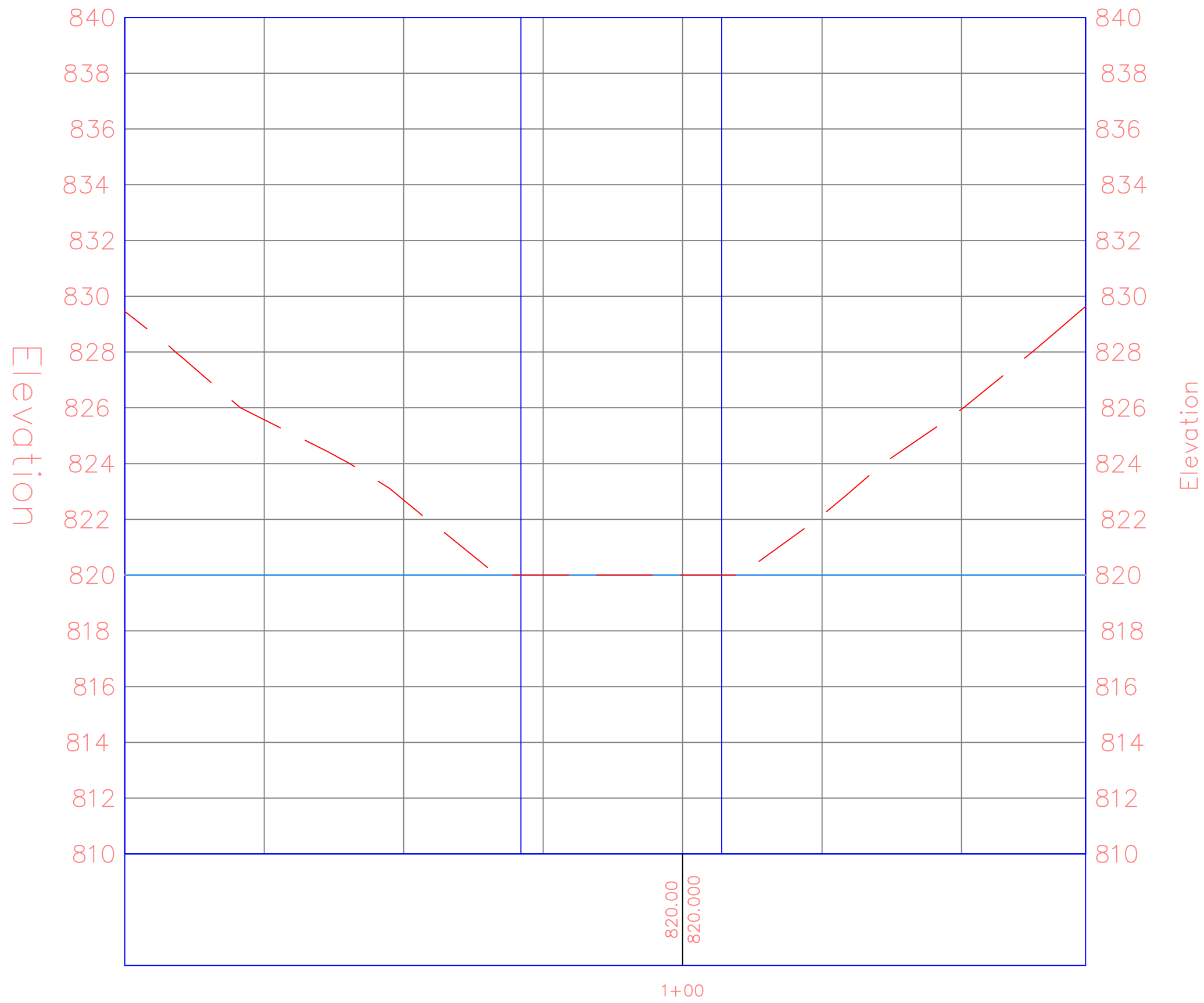
South Dock Loop PROFILE South Dock Loop61
