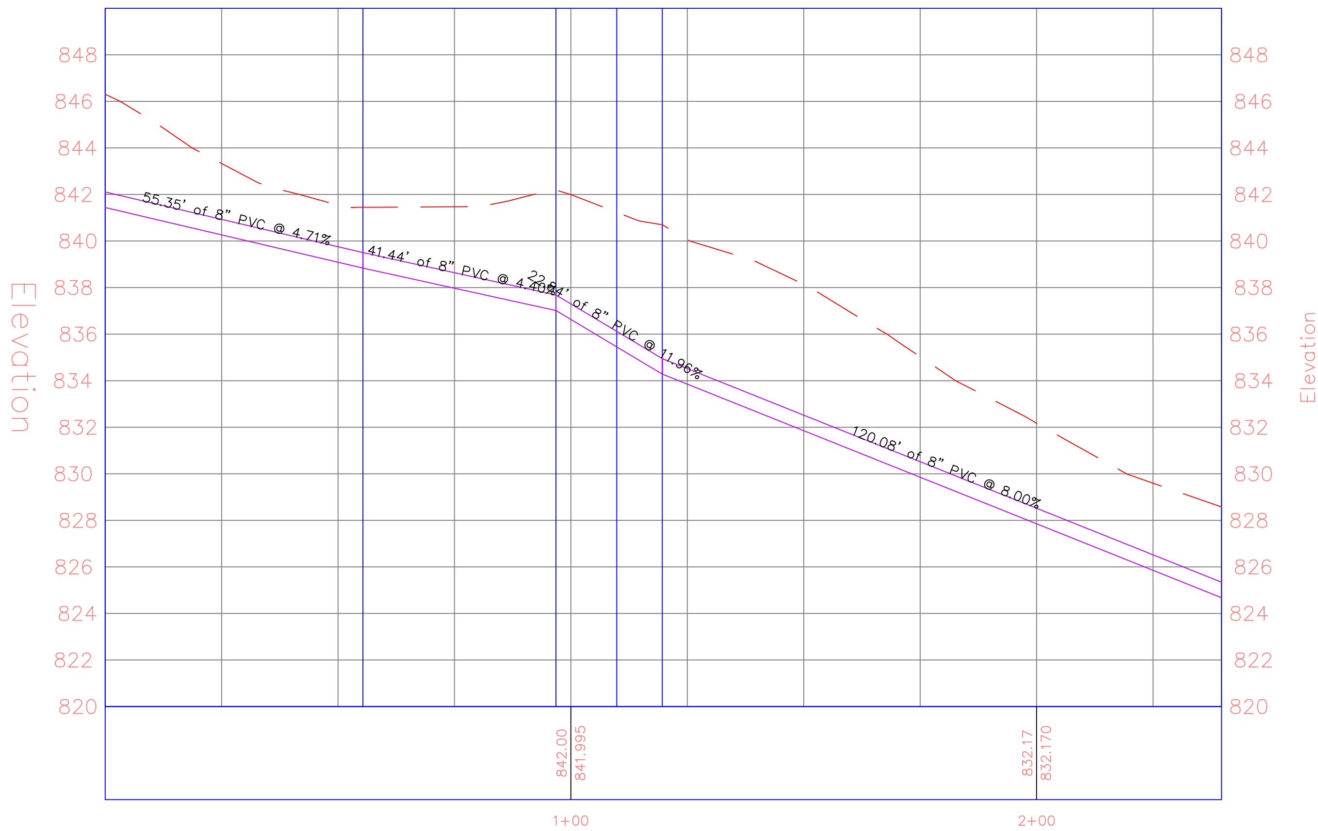
RV Dump Station PROFILE RV Dump SS86
