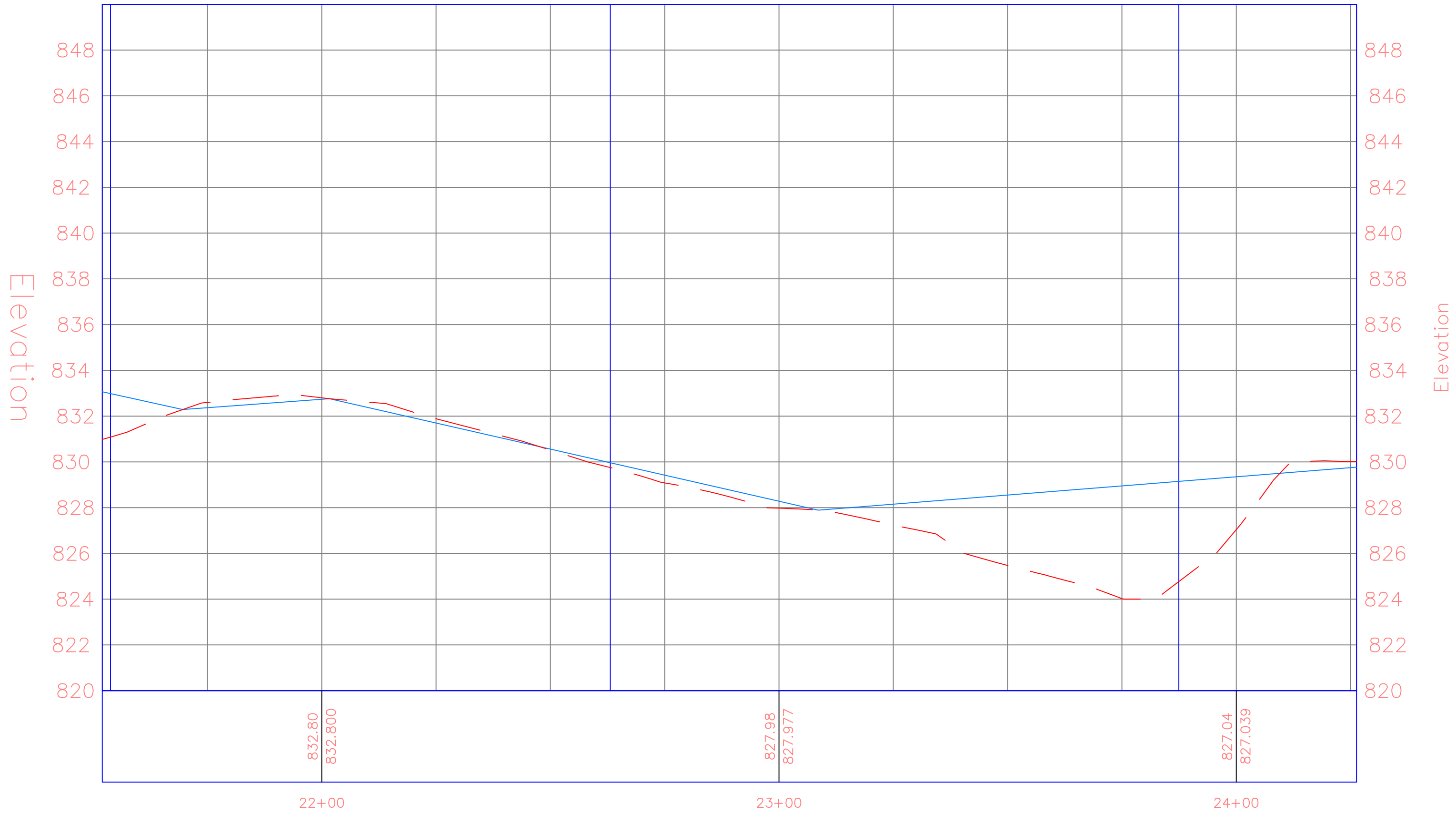
Gravel Path West PROFILE Gravel Path West57
