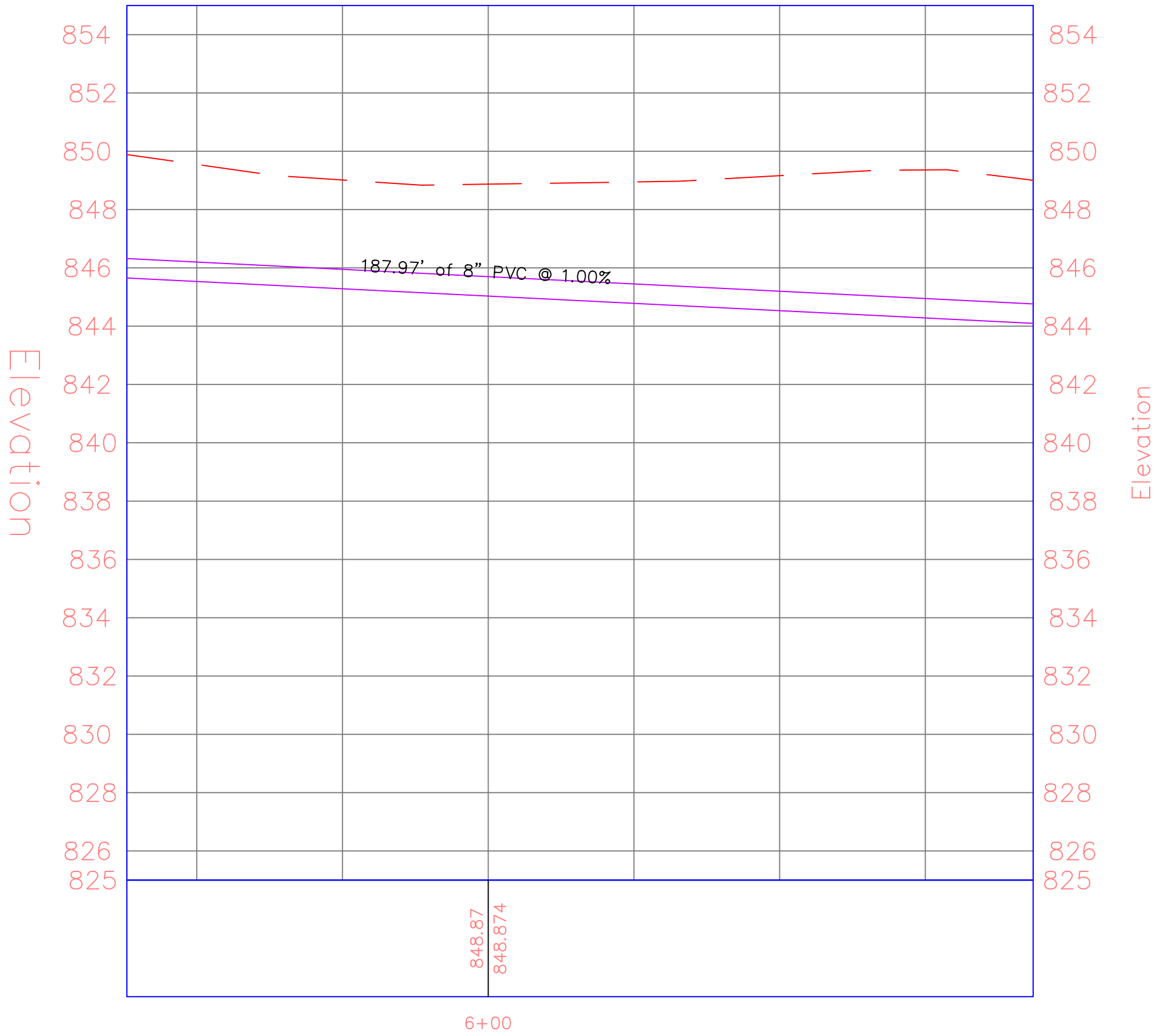
Venue Station Venue SS PROFILE Venue SS91
