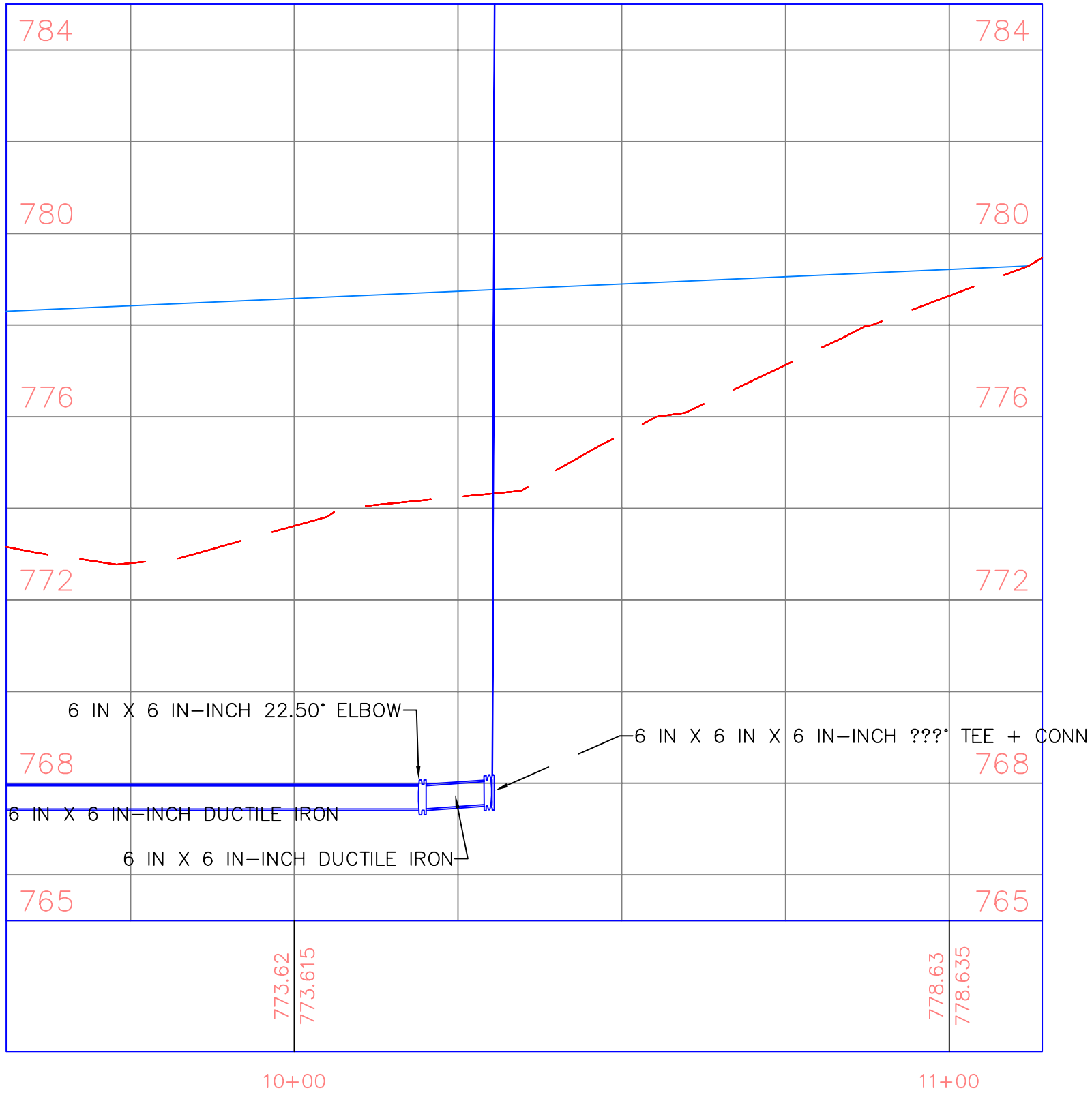
CL_ROAD PROFILE
